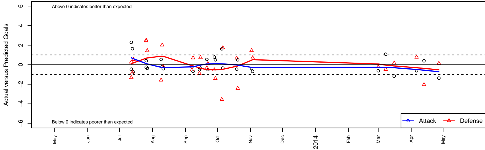
Crossfire OR LOSC Blue 2 G00 Dots are actual minus expected GF (blue circles) and GA (red triangles). Blue line is smoothed change in attack strength. Red is smoothed change in defense strength.
